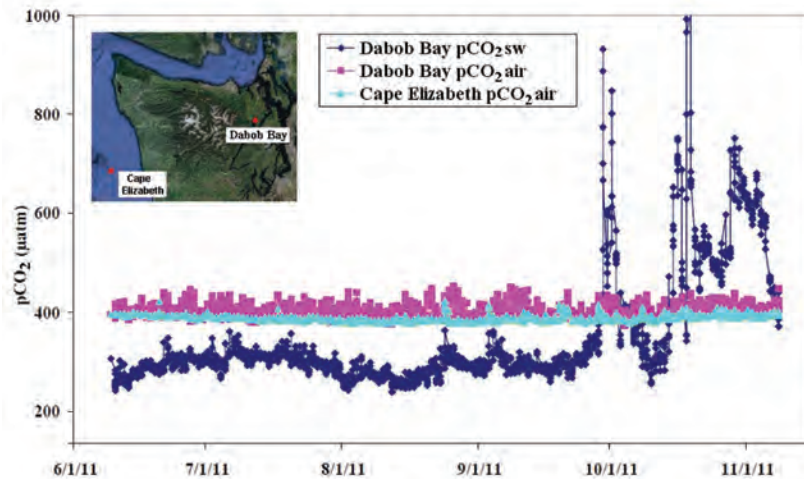
Figure 2.2 • Atmospheric pCO_2 (the partial pressure of CO_2 in units of \mu atm ) measurements by NOAA Pacific Marine Environmental Lab (PMEL) from the University of Washington buoy in Dabob Bay (in magenta) and NOAA National Data Buoy Center (NDBC) buoy off Cape Elizabeth on the outer Washington coast (in cyan). The surface seawater (sw) pCO_2 measurements at Dabob Bay are displayed in blue diamonds. The higher atmospheric pCO_2 values at Dabob Bay relative to the outer Washington Coast reflect the local sources of CO_2 in the atmosphere, which can enhance the summertime flux of carbon dioxide into the local waters by about 75%.
