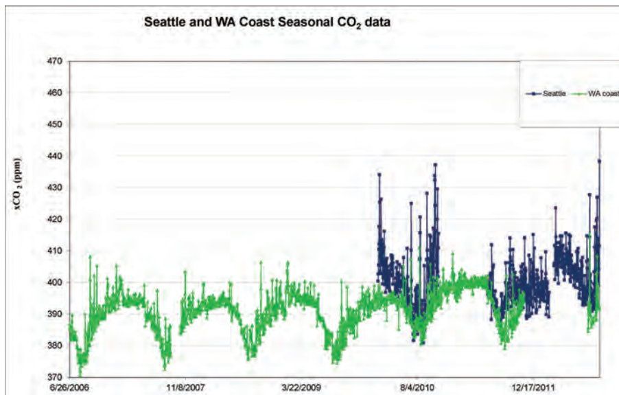
Figure 2.3 • Atmospheric xCO_2 (the mole fraction of CO_2 in units of ppm in dry air) measurements from NOAA PMEL for Seattle in blue (Space Needle) and the outer Washington coast in green (Cape Elizabeth NOAA NDBC buoy) showing full time record for coast (since 2006) and available data for Seattle (2010 and 2011). Note that the outer coast has an apparent upward trend with time. Graphics provided by Ellen Lettvin, Pacific Science Center; NOAA PMEL data exhibited in Pacific Science Center CO_2 kiosk and in collaboration with C. L. Sabine, NOAA PMEL.
