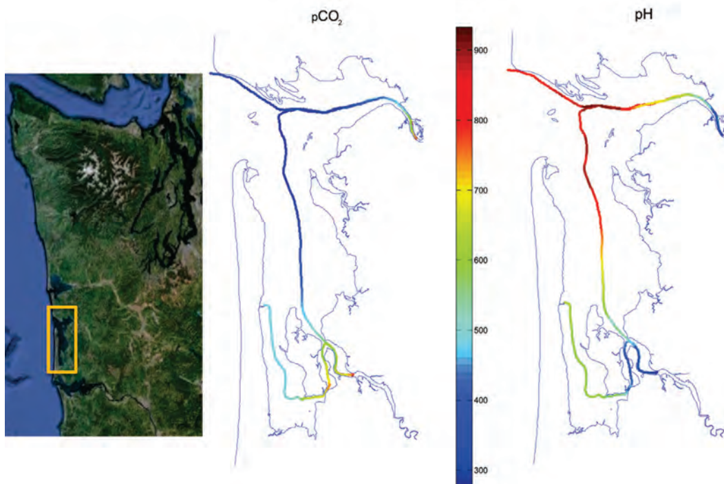
Figure 4.1 • Surface sampling for \text{pCO}_2 and pH measured during September 2010 in Willapa Bay. The survey, originating at Oysterville on the Long Beach Peninsula, has a survey arm in the southeast up the Naselle River estuary, then goes north and bifurcates with an arm to the east extending up the Willapa River estuary, and an arm to the west out to the Pacific Ocean. Funded by Washington Sea Grant, the UW study also documented watershed carbon inputs (Ruesink and Trimble, unpublished data ).
