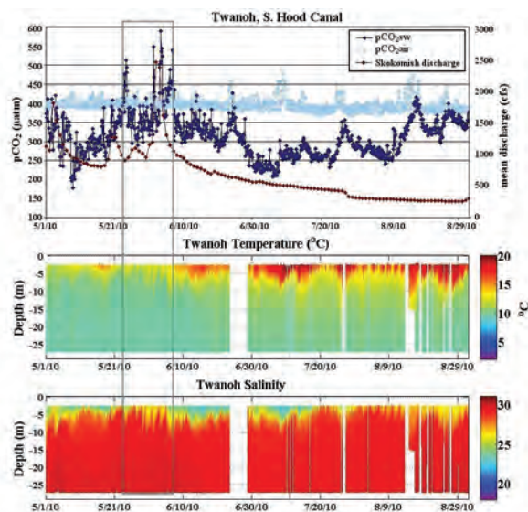
Figure 3.4 • Seasonal record of seawater and air \text{pCO}_2 from NOAA PMEL sensors on a NANOOS profiling buoy at Twanoh in S. Hood Canal. Also shown are the Skokomish River discharge (U.S. Geological Survey), and water column profiles of seawater temperature and salinity. Higher seawater \text{pCO}_2 coincides with destratification deep mixing events, as bounded by the grey box. The \text{CO}_2 data are courtesy C. L. Sabine (NOAA PMEL); oceanographic data are courtesy A. Devol and J. Newton (UW).
